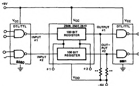
100-BIT DELAY
