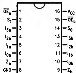
Pin Assignment for DIP, Flatpak and SOIC
