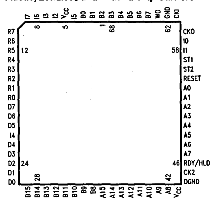
Plastic, Leadless and Leaded Chip Carriers
