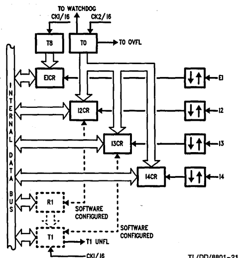
FIGURE 15. Timers T0, T1 and T8 with Four Input Capture Registers
