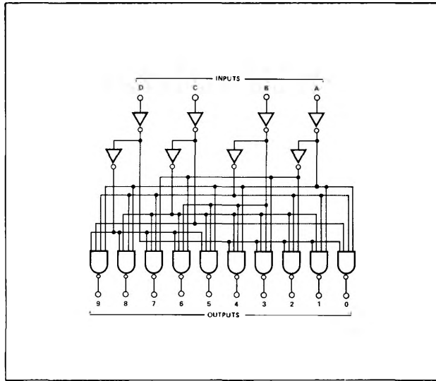
S5444/N7444 EXCESS 3 GRAY INPUT
