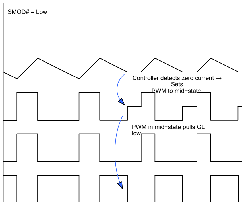
Figure 16. Timing Diagram – 3-state PWM Controller, with ZCD
