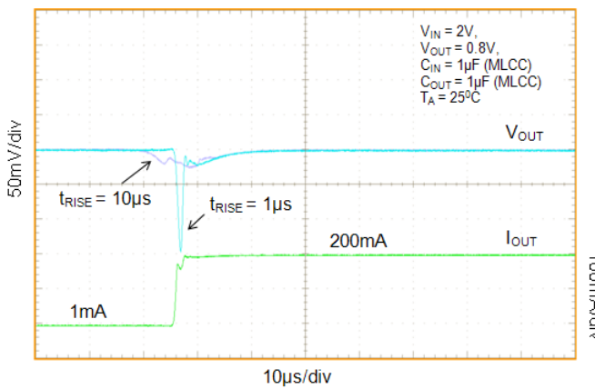
Figure 49. Load Transient Response – Rising Edge, I_{OUT} = 1\text{ mA} - 200\text{ mA} , C_{OUT} = 1.0\text{ }\mu\text{F}
