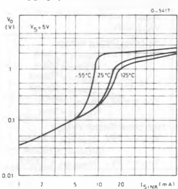
Figure 4 : Low Output Voltage Vs. Output Sink Current.
