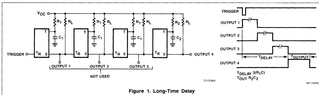
Figure 1. Long-Time Delay
