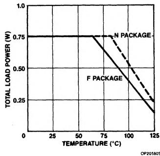
Total Load Power vs Temperature (NE590)
