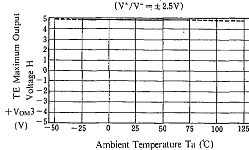
TE Maximum Output Voltage H vs. Temperature
