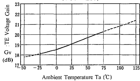
TE Voltage Gain vs. Temperature
