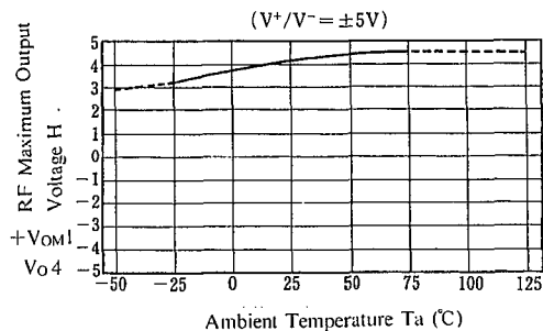
RF Maximum Output Voltage H vs. Temperature
