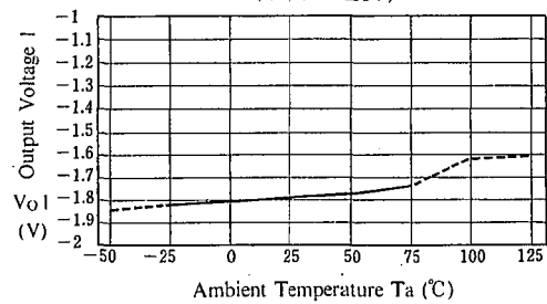
APC Vo1 vs. Temperature
