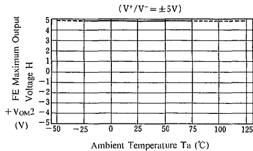
FE Maximum Output Voltage H vs. Temperature
