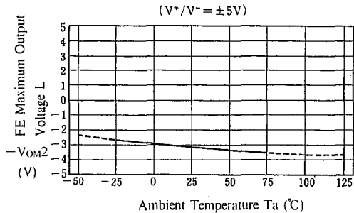
FE Maximum Output Voltage L vs. Temperature
