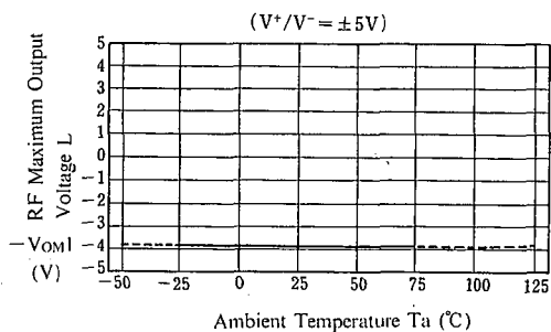
RF Maximum Output Voltage L vs. Temperature
