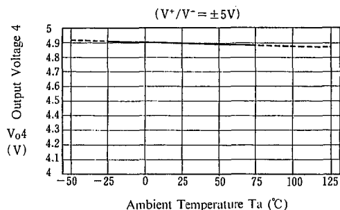
APC Vo4 vs. Temperature
