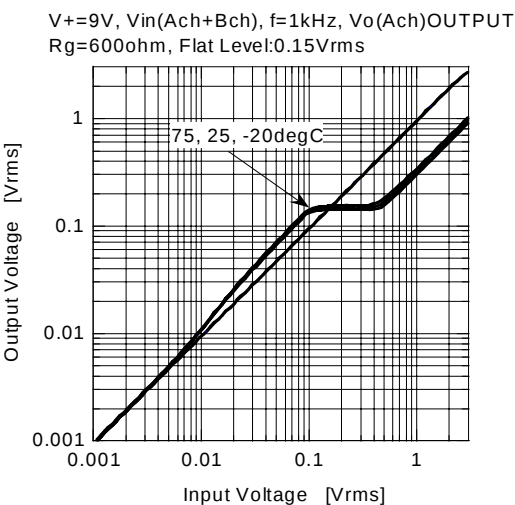
AGC Control
