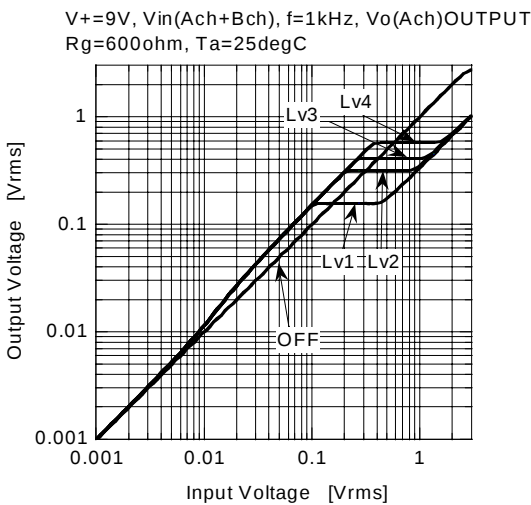
AGC Control
