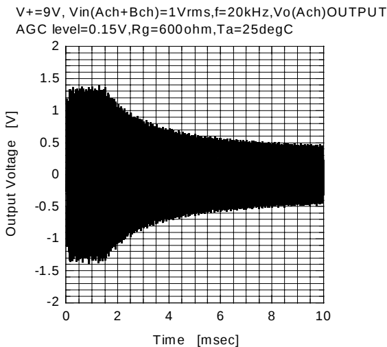
AGC Attack Time
