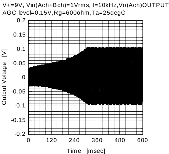
AGC Recovery Time
