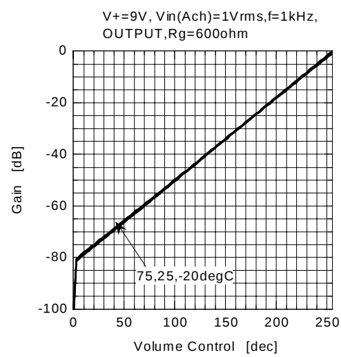
Gain vs Volume Control
