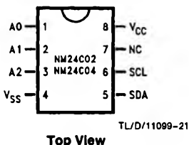
SO Package (M8)
