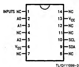
SO Package (M)
