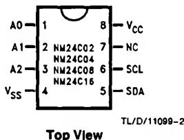
Dual-In-Line Package (N)
