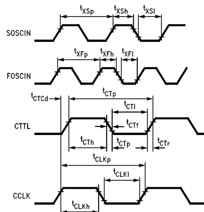
FIGURE 4-8. Clock Waveforms
