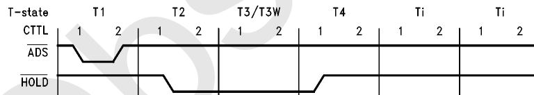
FIGURE 3-20. Spaced Memory Transaction, Two Tidles after T4
