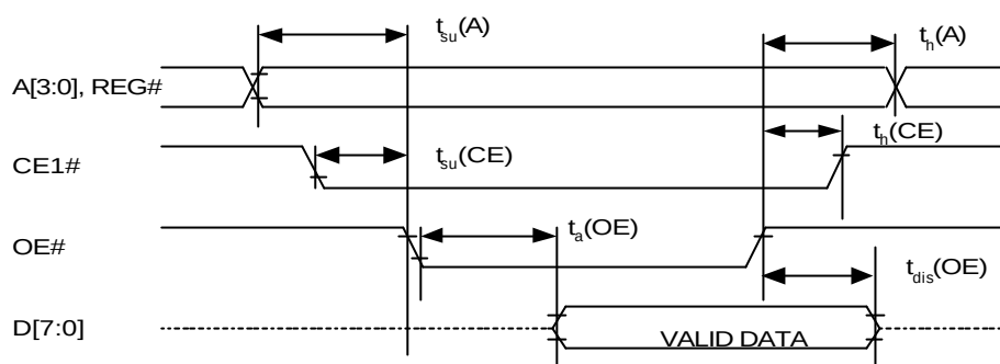
Figure 8: Attribute/Common Memory Read Timing
