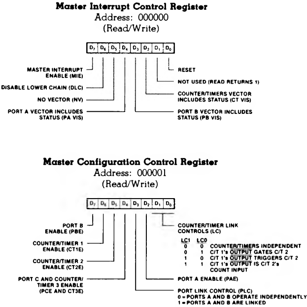
Figure 12. Master Control Registers
