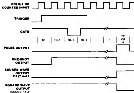
Figure 10. Counter/Timer Waveforms
