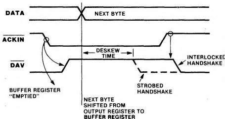
Figure 7. Interlocked and Strobed Handshakes
