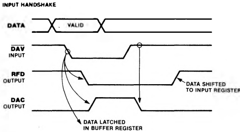
Figure 8. 3-Wire Handshake
