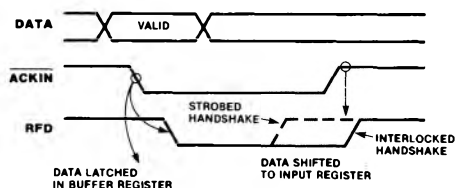
Figure 7. Interlocked and Strobed Handshakes
