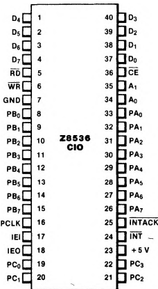
Figure 2. Pin Configurations
