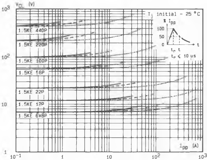
Fig.2 - Clamping voltage versus peak pulse current. exponential waveform t = 20 μs ..... t = 1 ms ---- t = 10 ms ———
