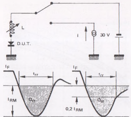
FIGURE 12 : Measurement of t_{rr} (fig. 9) and I_{RR} (fig. 10)
