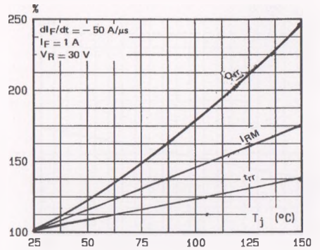
Fig. 9 - Dynamic parameters versus junction temperature.
