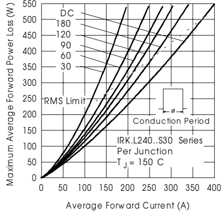
Fig.10-ForwardPowerLossCharacteristics
