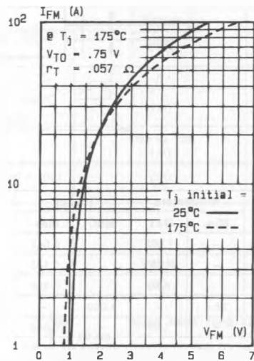
Fig. 7 - Peak forward current versus peak voltage drop (typical values for unidirectional types).
