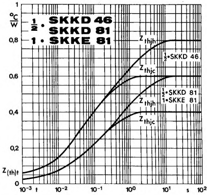
Fig. 14 Transient thermal impedance vs. time
