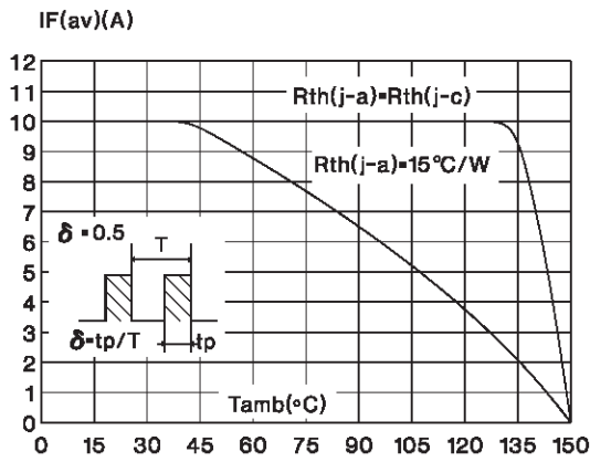
Fig. 2-1: Average current versus ambient temperature ( \delta : 0.5 ) (TO-220AC).
