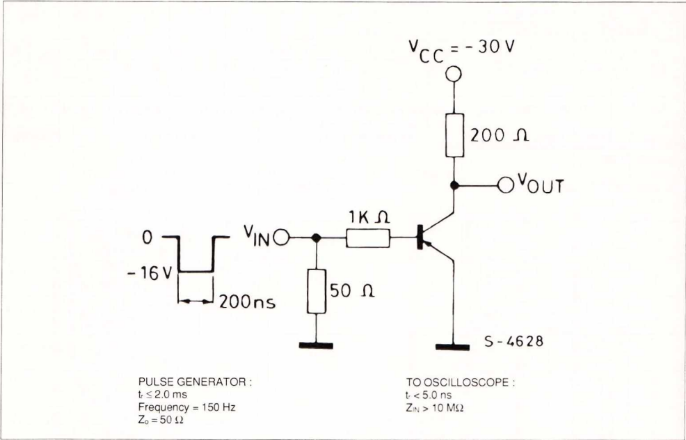
Test Circuit for t_{off} , t_b , t_r .
