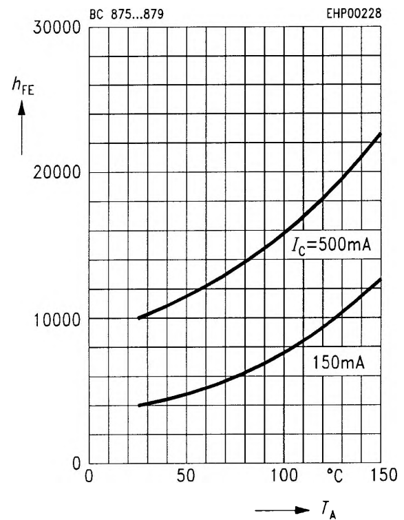
DC current gain h_{FE} = f(T_A) V_{CE} = 10 V
