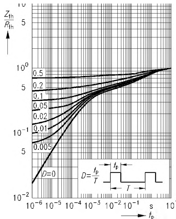
Permissible pulse load r_{thJA} = f(t_p) normalized
