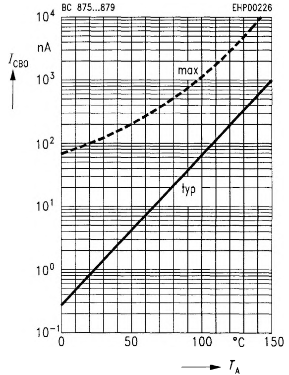
Collector cutoff current I_{CB0} = f(T_A) V_{CB} = 100 V
