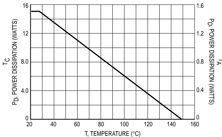
Figure 1. Power Derating
