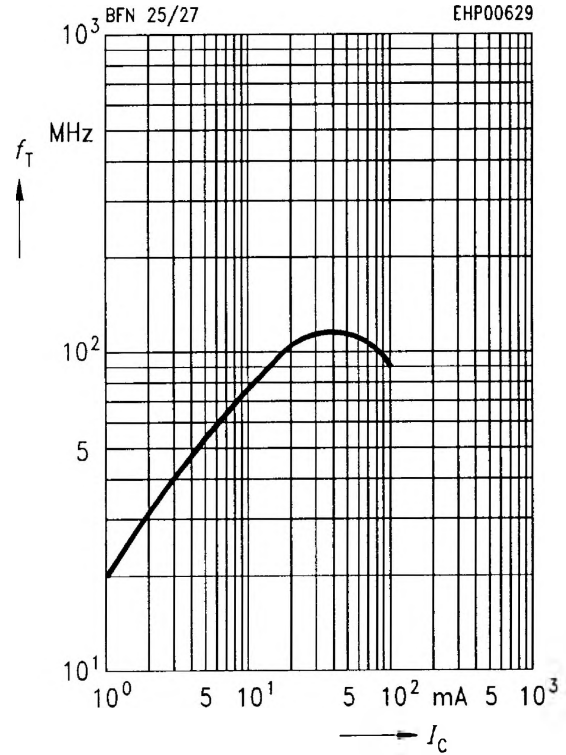
Transition frequency f_T = f(I_C) V_{CE} = 10 V
