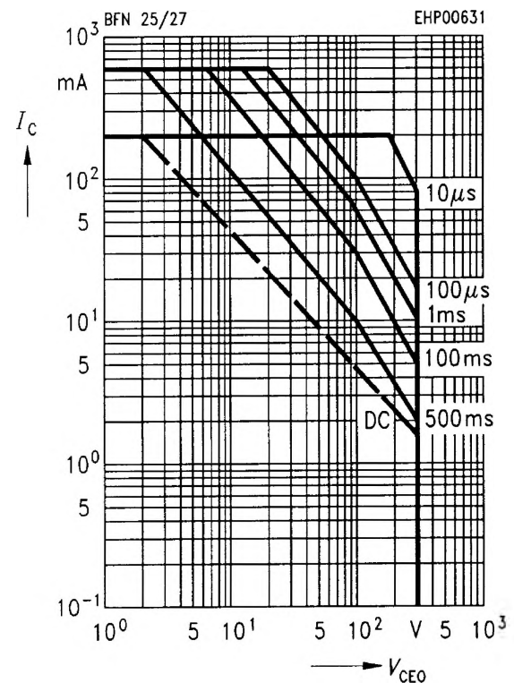
Operating range I_C = f(V_{CE0}) T_A = 25 °C, D = 0
