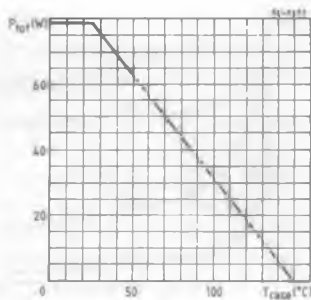
Derating curve
