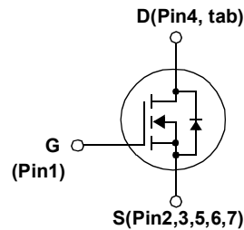
D 2 -PAK-7L FDB Series with suffix - L7
