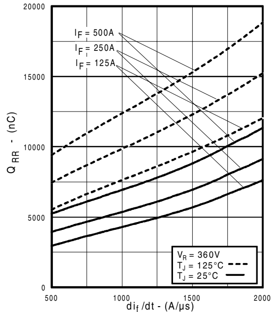
Fig. 14 - Typical Stored Charge vs. di_i/dt
