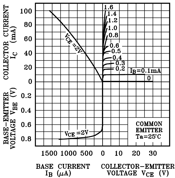
STATIC CHARACTERISTICS
