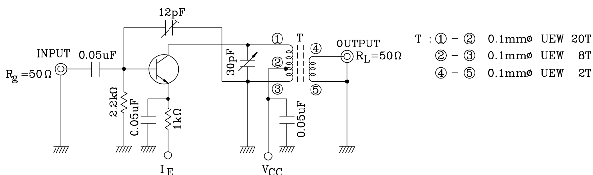
Fig. G_{pe} TEST CIRCUIT
