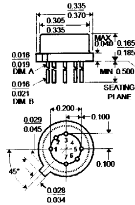
TO-78
