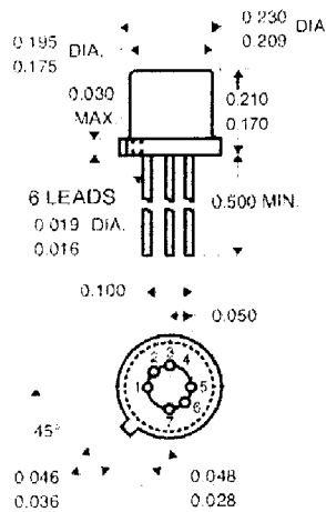
TO-71 Six Lead
