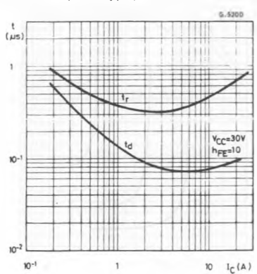
Turn-on Time (PNP type).
