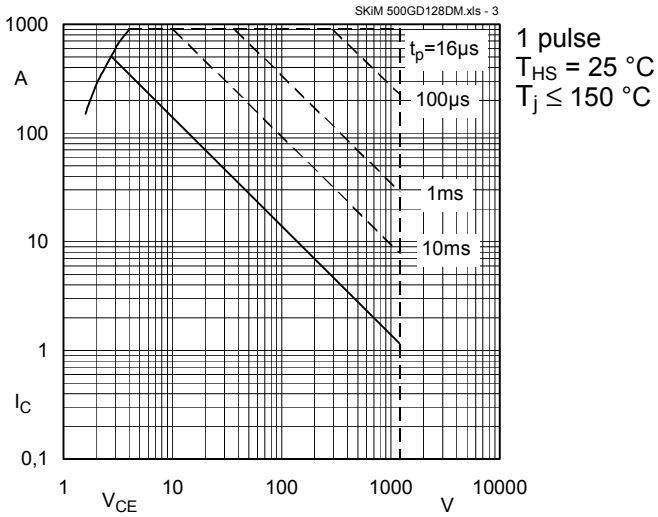
Fig. 3 Maximum safe operating area (SOA) I_C = f (V_{CE})
