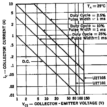
Maximum Safe Operating Area U2T101 & 105
