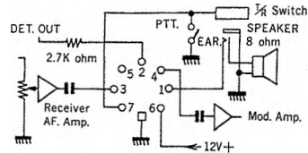
6. Internal connection
