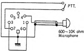
3. External microphone
